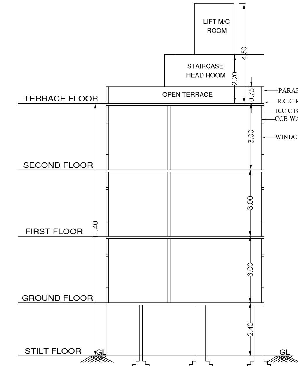
SECTION @ 'A'-'A'
